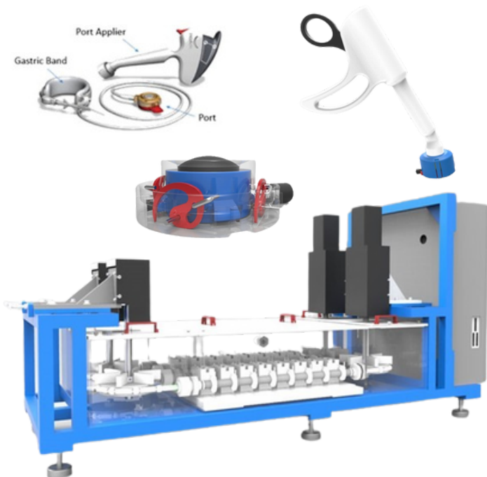
Gastric Band Test Machine
